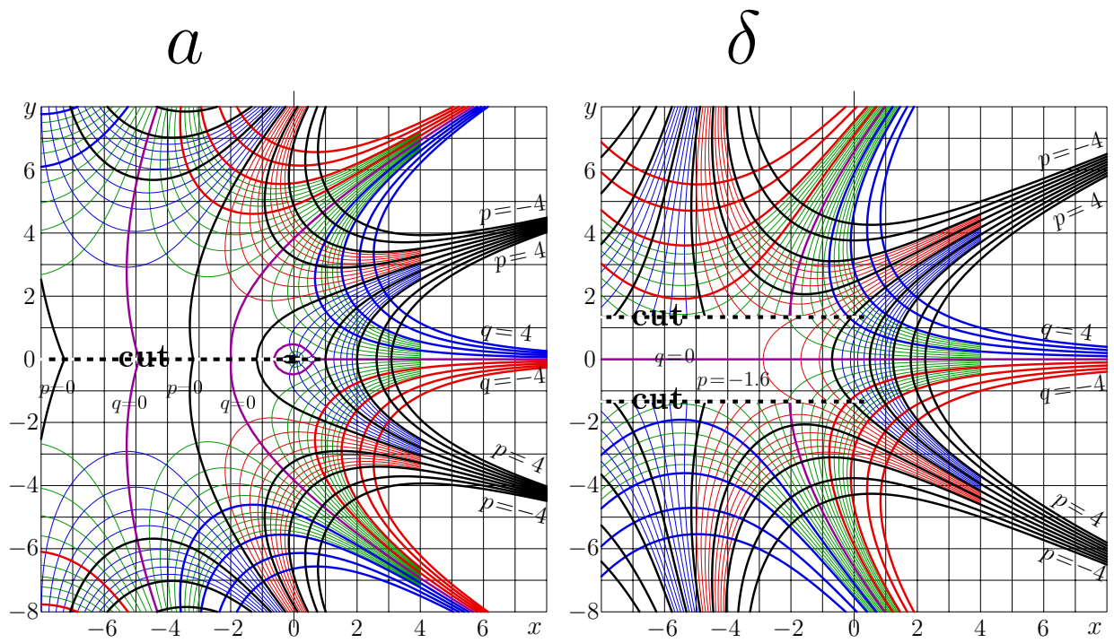
Рис. 5: f = \sqrt{\Gamma}(z) = \text{Factorial}^{-1/2}(z) by (11), left, and f = \sqrt{\exp}(z) , right, in the complex z -plane in the same notations as in figures 3, 4
