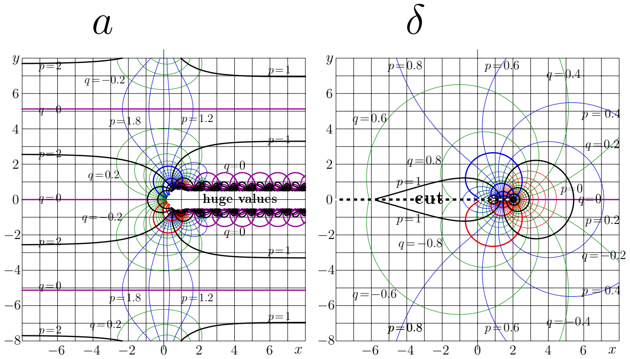
Рис. 4: Maps of F and G in the same notations as in figure 3.
