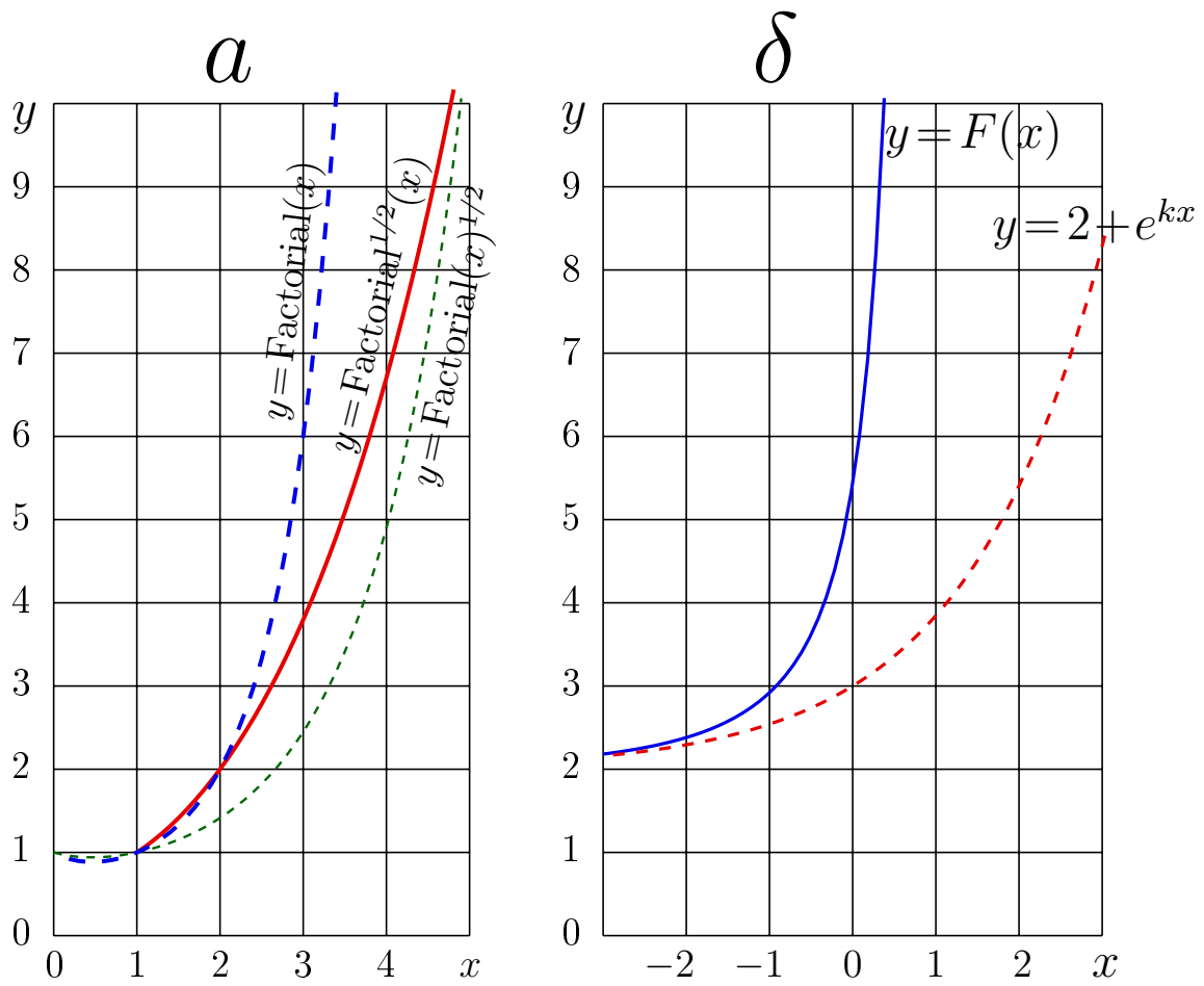
Рис. 2: Left: y = \text{Factorial}(x) , thick dashed curve; y = \sqrt{x!} = \text{Factorial}^{1/2}(x) , solid curve; y = \sqrt{x!} = \text{Factorial}(x)^{1/2} , thin dashed, as functions of real x ; Right: y = F(x) , solid, compared to y = 2 + \exp(kx) , dashed
