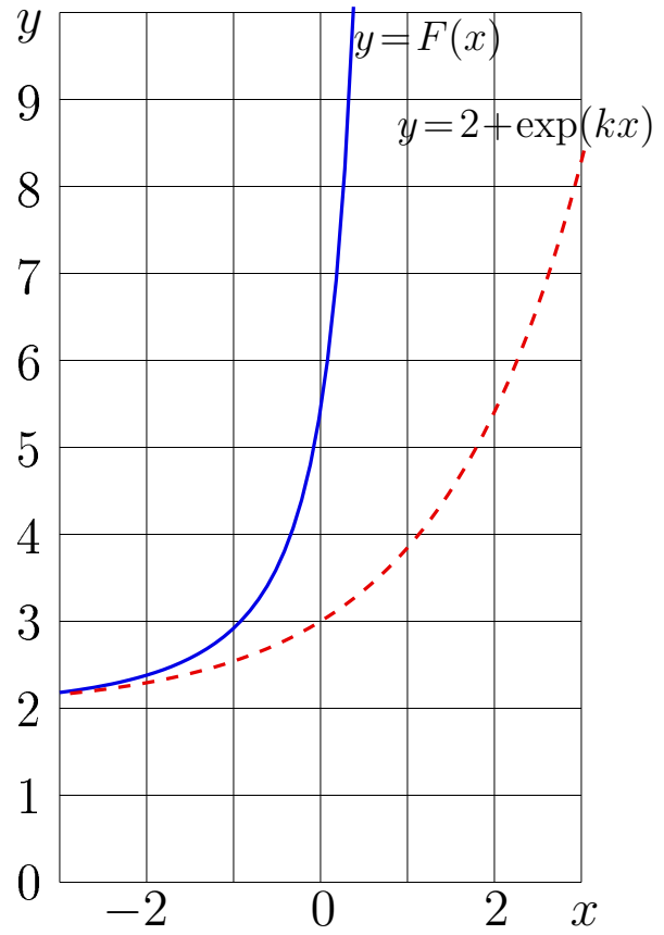
FIG. 1: Left: y = \text{Factorial}(x) , thick dashed curve; y = \sqrt{x!} = \text{Factorial}^{1/2}(x) , solid curve; y = \sqrt{x!} = \text{Factorial}(x)^{1/2} , thin dashed, as functions of real x ; Right: y = F(x) , solid, compared to y = 2 + \exp(kx) , dashed
