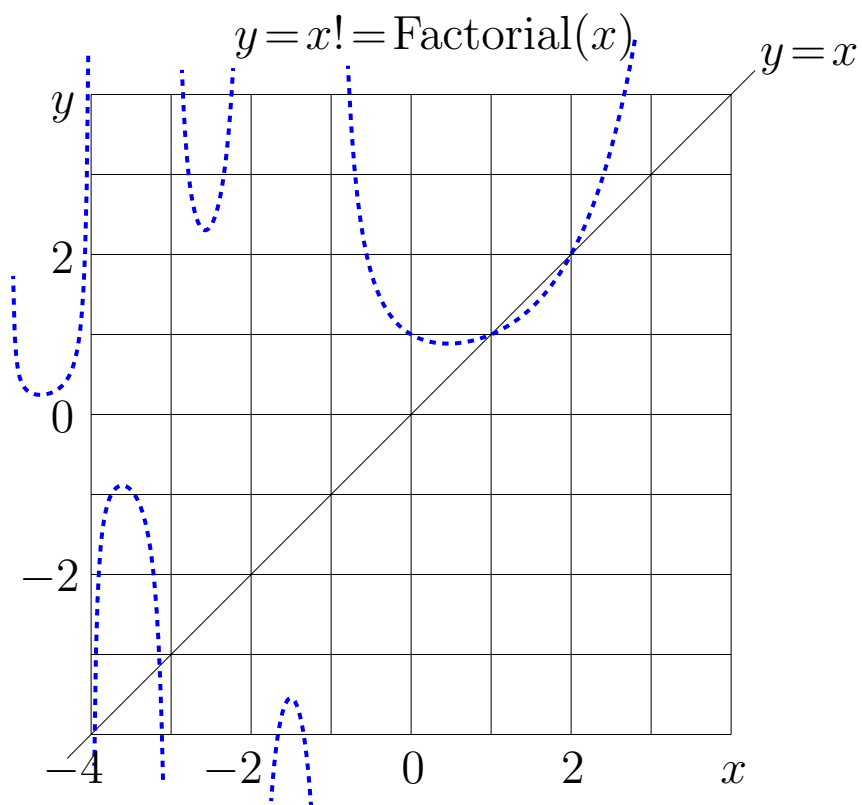
Рис. 0: Factorial of the real argument and graphical solution of equation x! = x .
