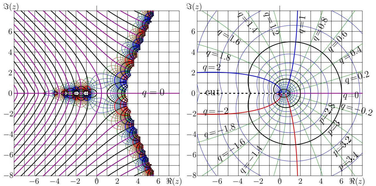
Рис. 2: f = \text{Factorial}(z) , left, and f = \text{ArcFactorial}(z) , right, in the complex z -plane; Levels \Re(f) = p = \text{constant} and Levels \Im(f) = q = \text{constant} are shown with thick lines for p = -4, -3, -2, -1, 0, 1, 2, 3, 4 and for q = -4, -3, -2, -1, 0, 1, 2, 3, 4
