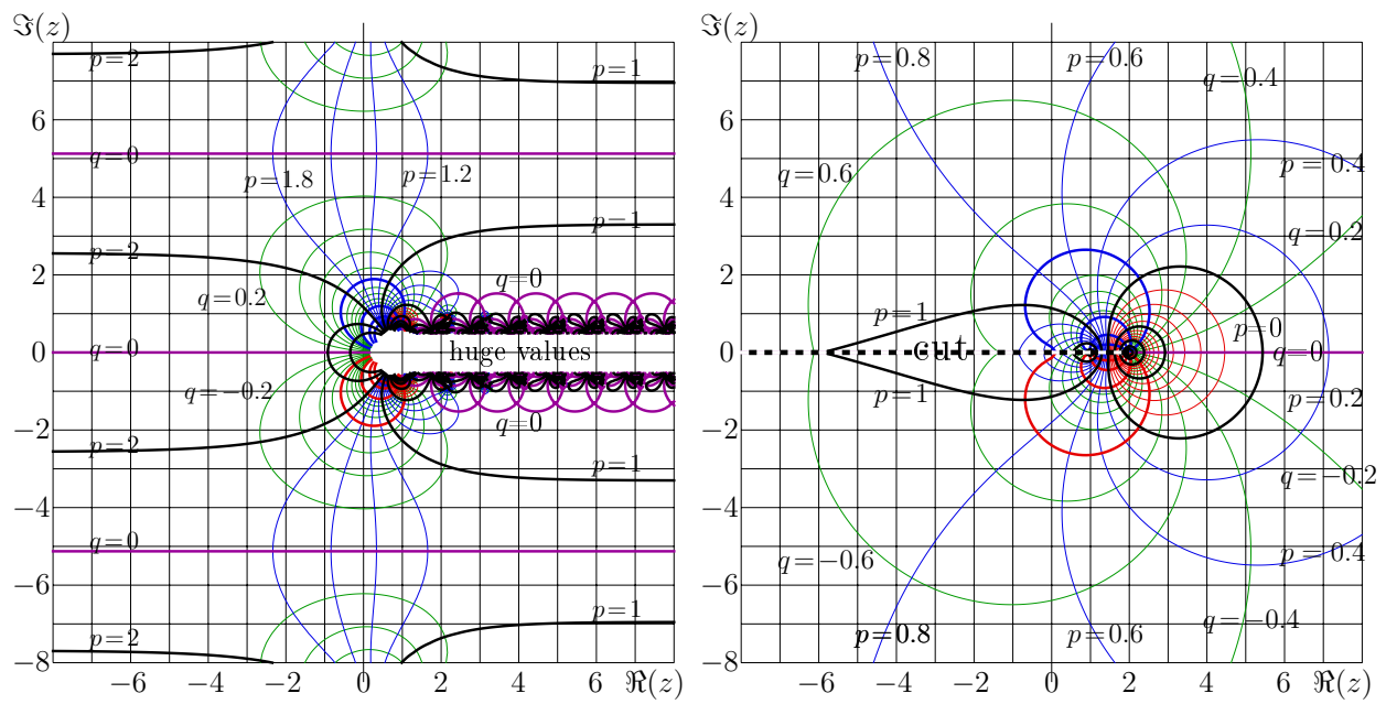
Рис. 3: Maps of F and G in the same notations as in figure 2.
