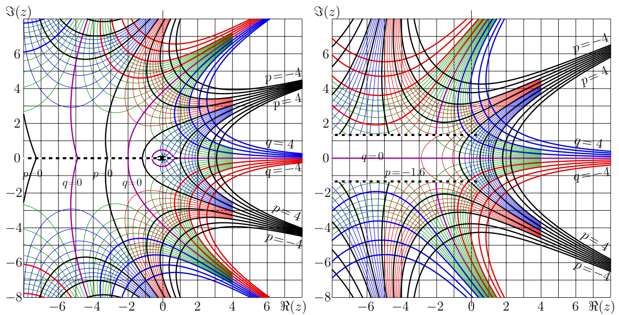
Рис. 4: f = \sqrt{1(z)} = \text{Factorial}^{-1/2}(z) by (10), left, and f = \sqrt{\exp(z)} , right, in the complex z -plane in the same notations as in figures 2, 3
