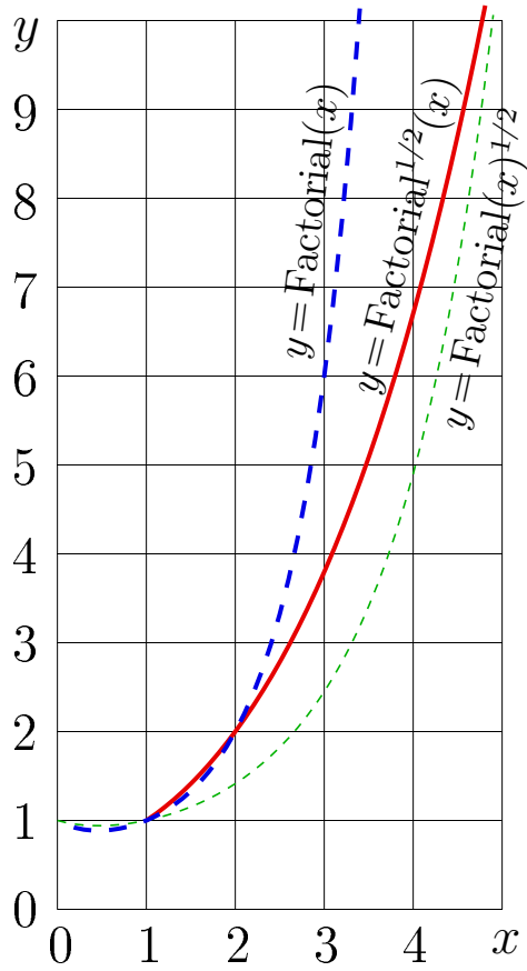
FIG. 1: Left: y = \text{Factorial}(x) , thick dashed curve; y = \sqrt{x!} = \text{Factorial}^{1/2}(x) , solid curve; y = \sqrt{x!} = \text{Factorial}(x)^{1/2} , thin dashed, as functions of real x ; Right: y = F(x) , solid, compared to y = 2 + \exp(kx) , dashed
