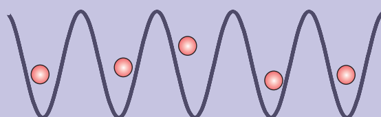
Optical Lattice
