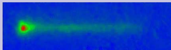
Atom Laser
