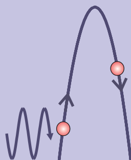
Atomic Clock
